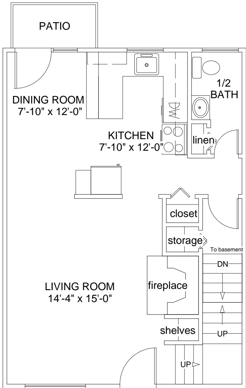
1st Floor
